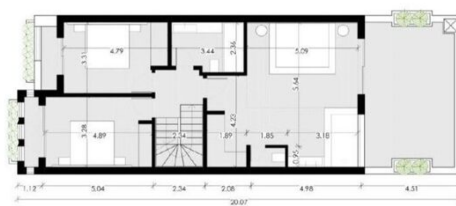
LEVEL 01
